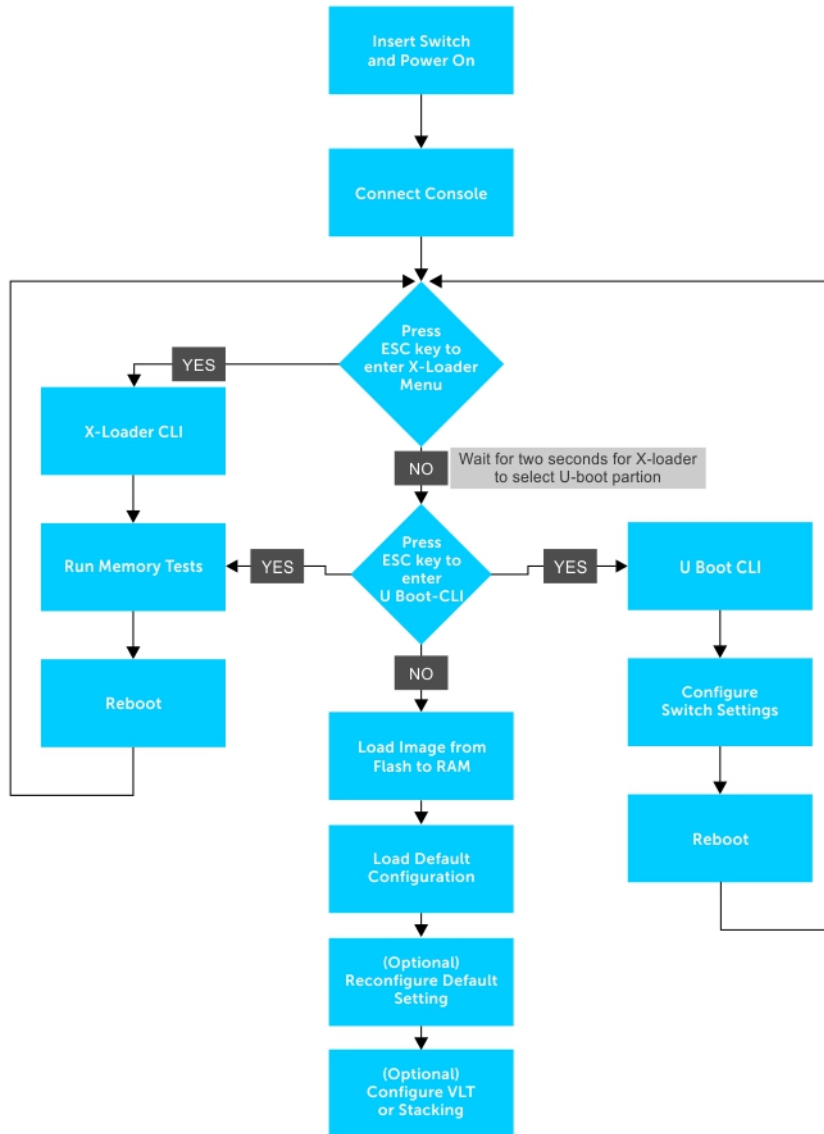
Figure 3. Aggregator — Installation and Configuration Flowchart
