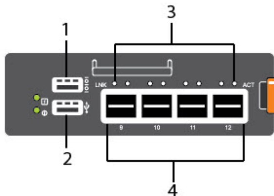
Figure 1. I/O Panel
